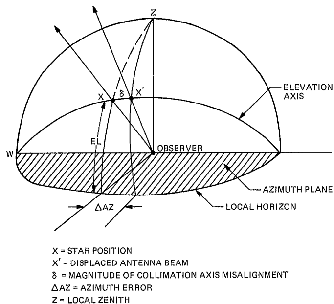
Fig. 3. Azimuth collimation error
