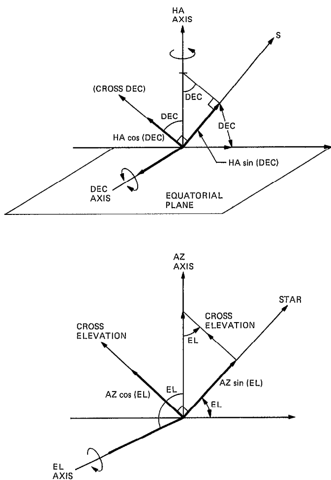
Fig. 2. Azimuth-elevation and hour-angle declination coordinate systems showing cross elevation and cross-declination axes, respectively
