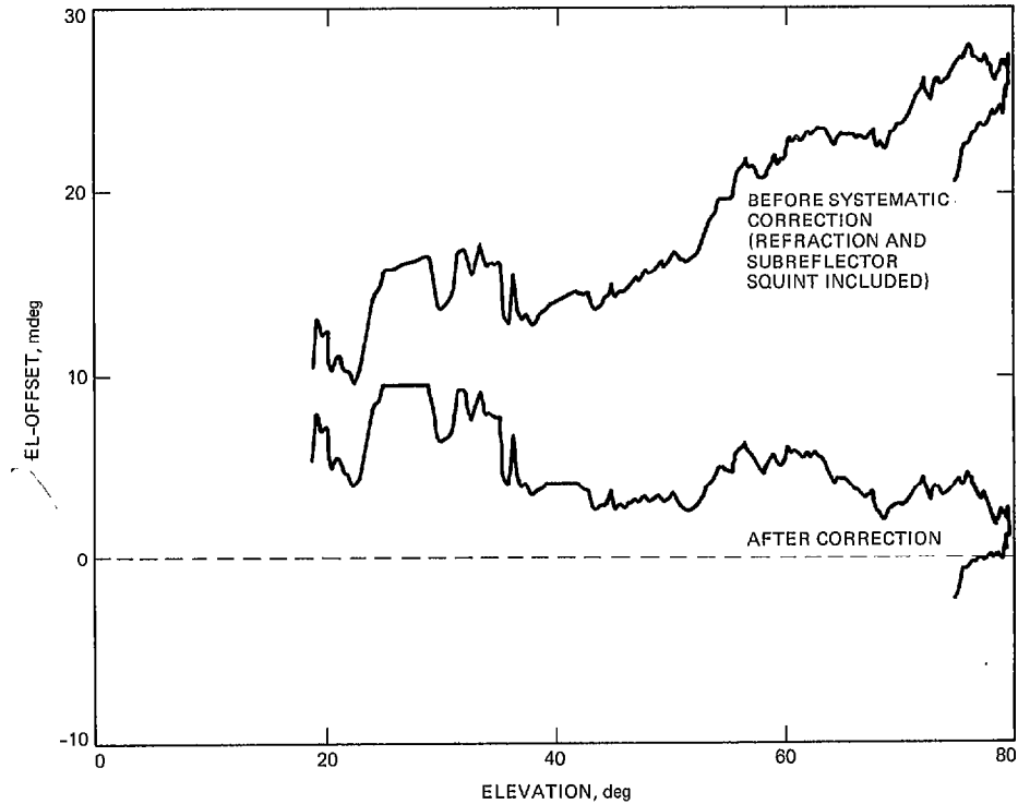
Fig. 7. Elevation vs EL-offset before and after systematic error correction, Mars, 64-m antenna
